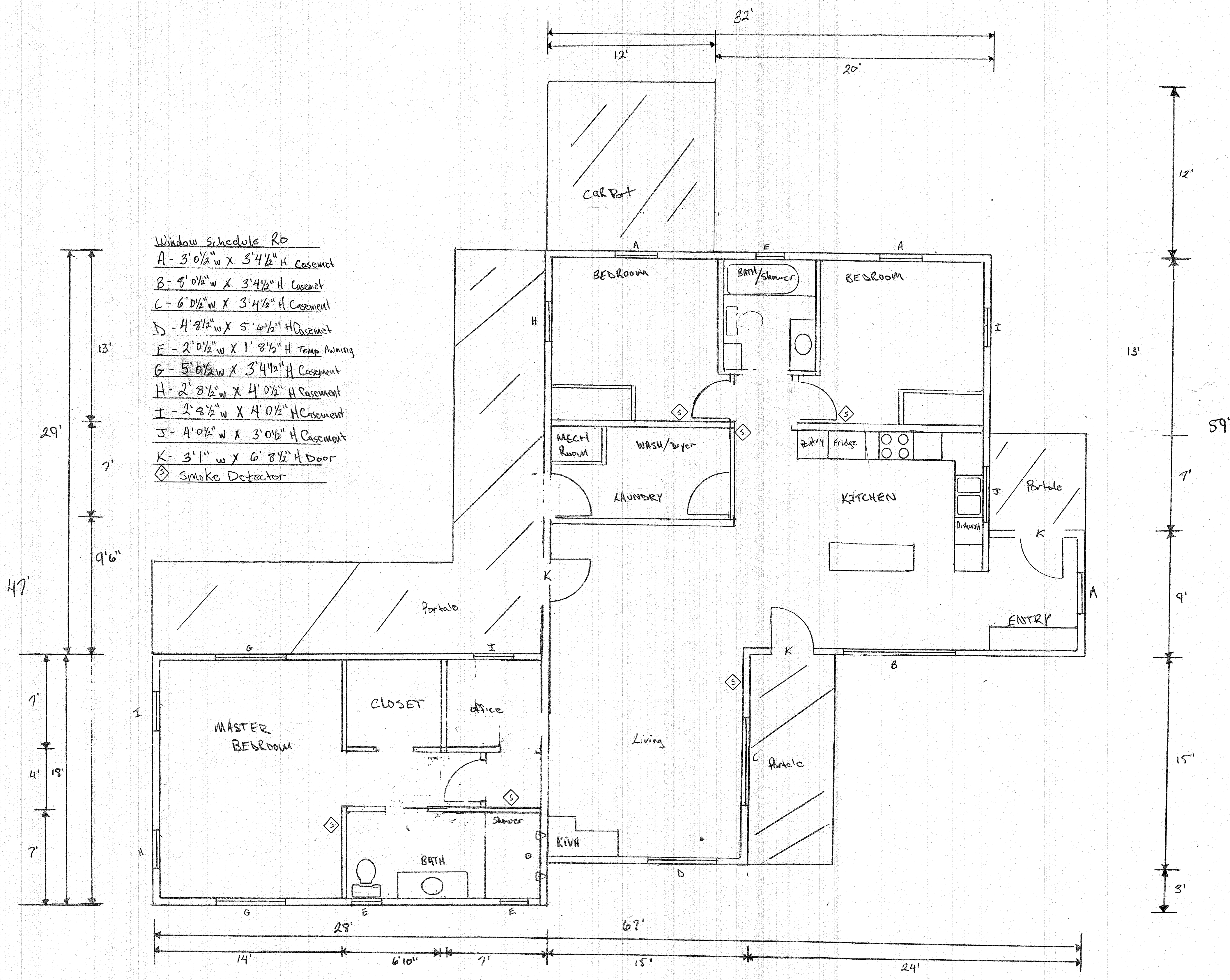
Floor Plan 1/4" = 1'
